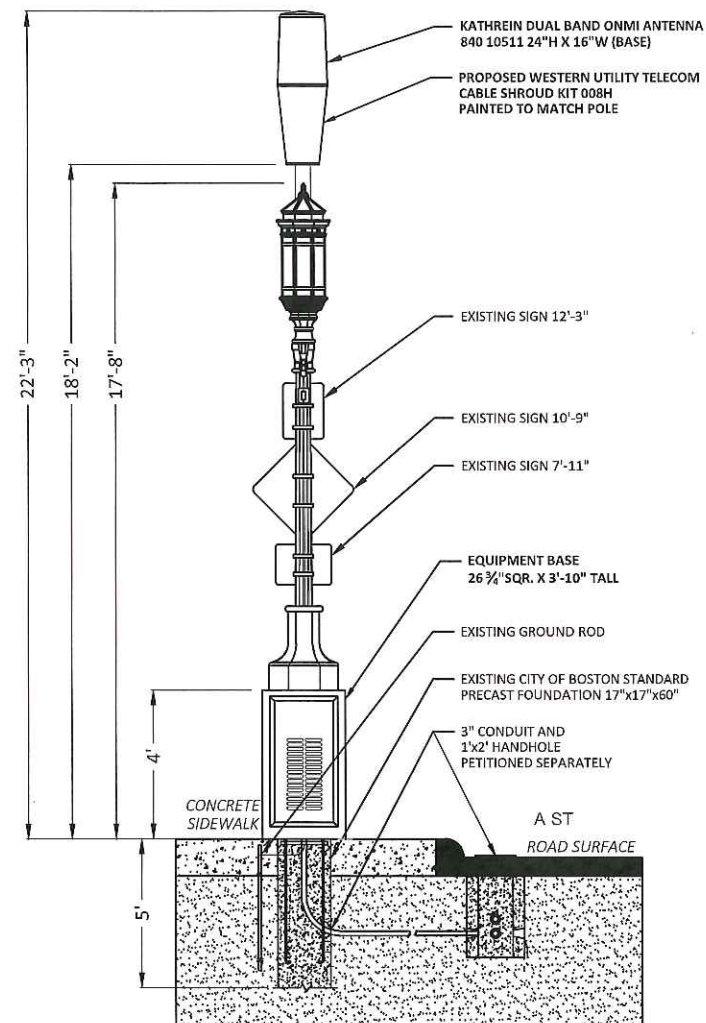
POLE DIAGRAM SIDE VIEW
