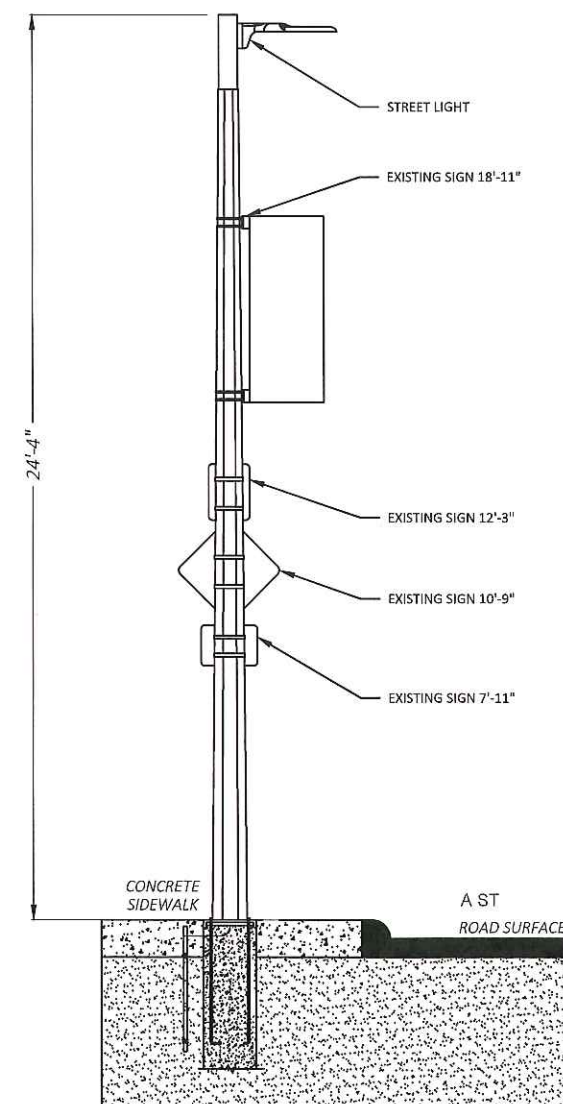
POLE DIAGRAM SIDE VIEW
