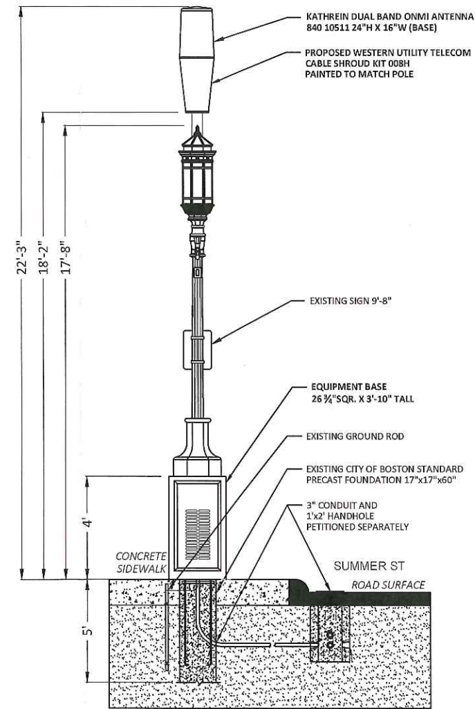
POLE DIAGRAM SIDE VIEW
