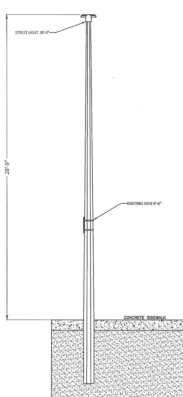
POLE DIAGRAM REAR VIEW
