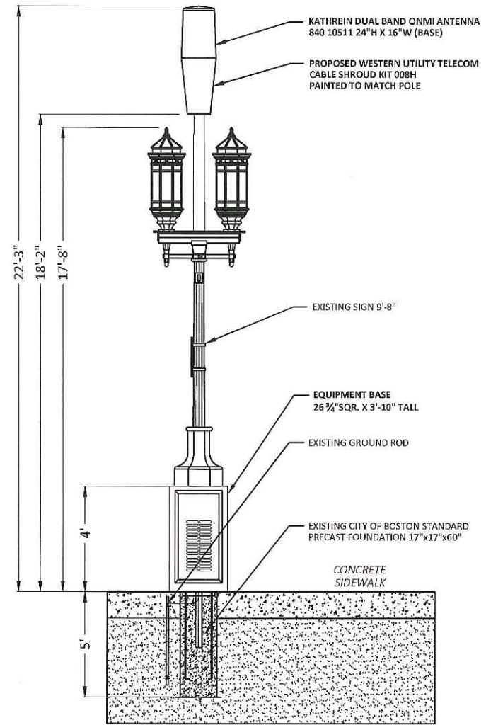
POLE DIAGRAM REAR VIEW
