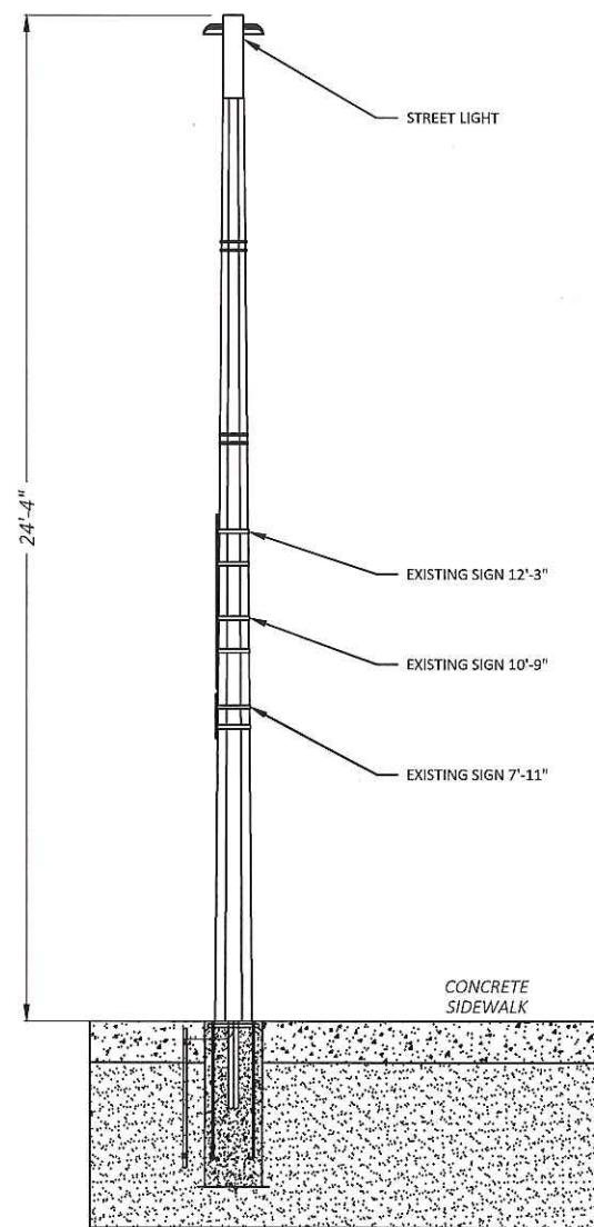
POLE DIAGRAM REAR VIEW
