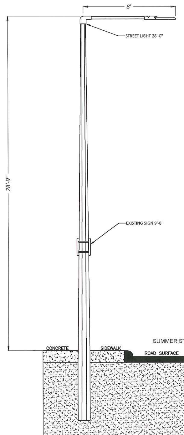
POLE DIAGRAM SIDE VIEW
