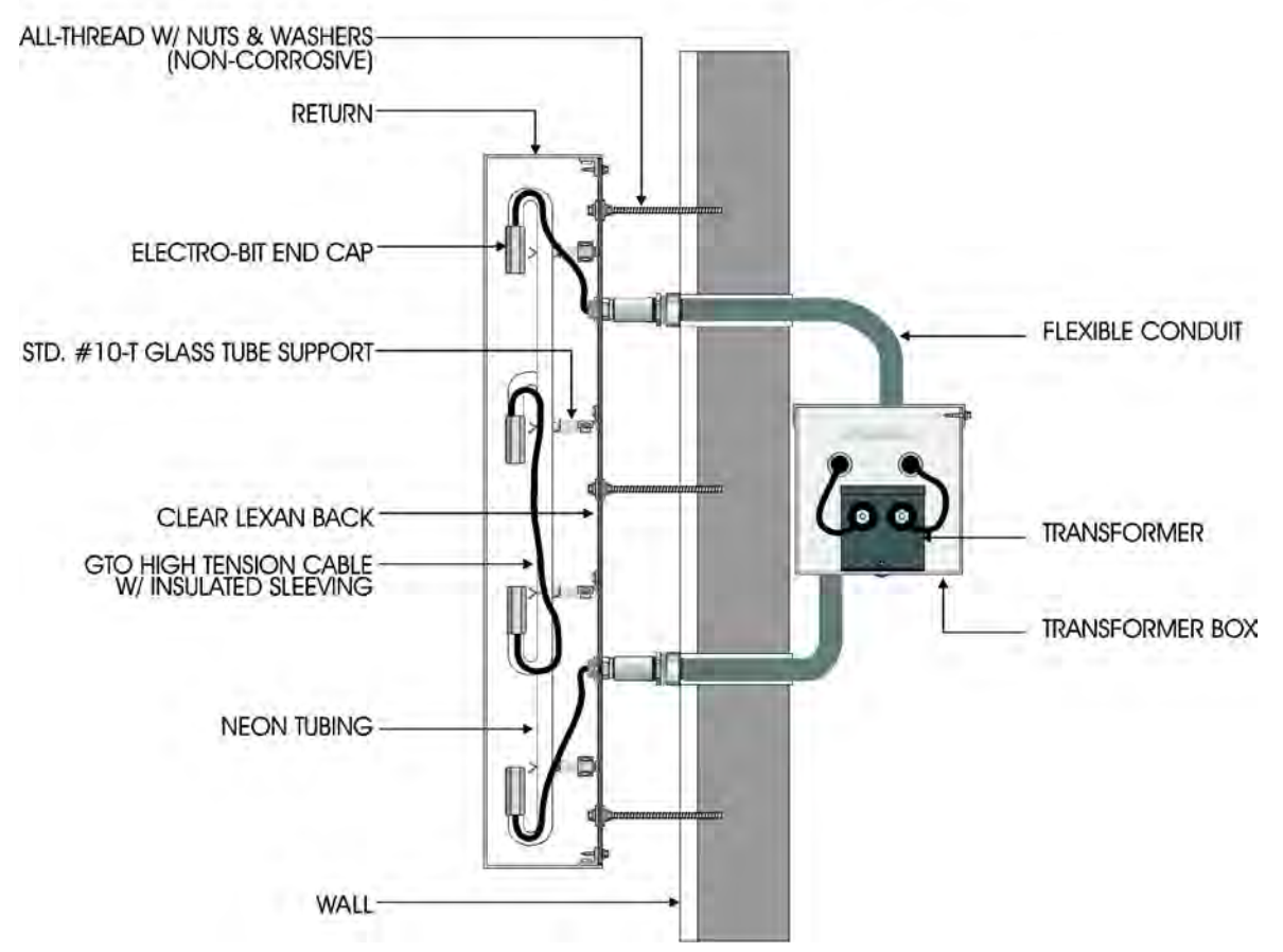
3 Letter Mounting Detail
