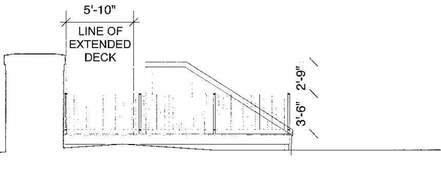
12 PROPOSED NORTH ELEVATION 1/8" = 1'-0"
