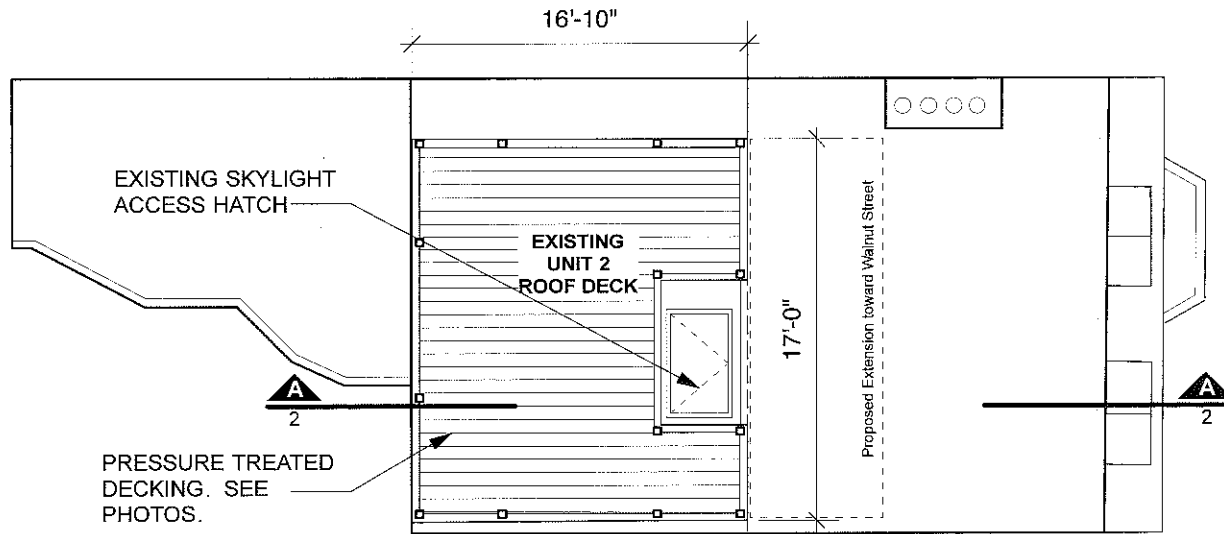
1 EXISTING ROOF PLAN 1/8" = 1'-0"
