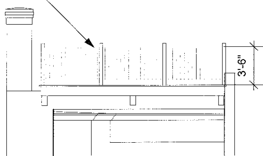
9 EXISTING WEST ELEVATION (REAR) 1/8" = 1'-0"
