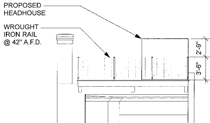
13 PROPOSED WEST ELEVATION (REAR) 1/8" = 1'-0"
