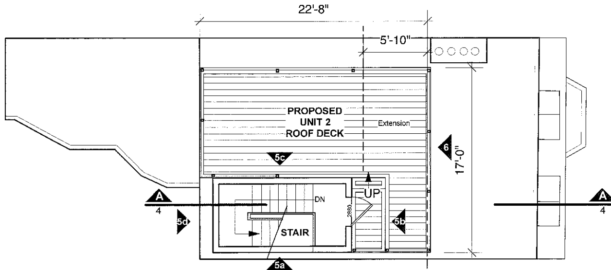
3 PROPOSED ROOF PLAN 1/8" = 1'-0"
