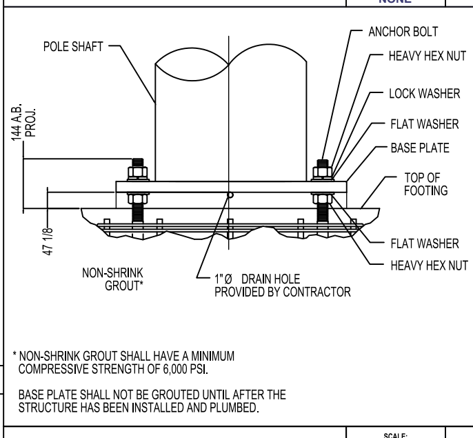
BASE GROUTING DETAIL SCALE: NONE 3
