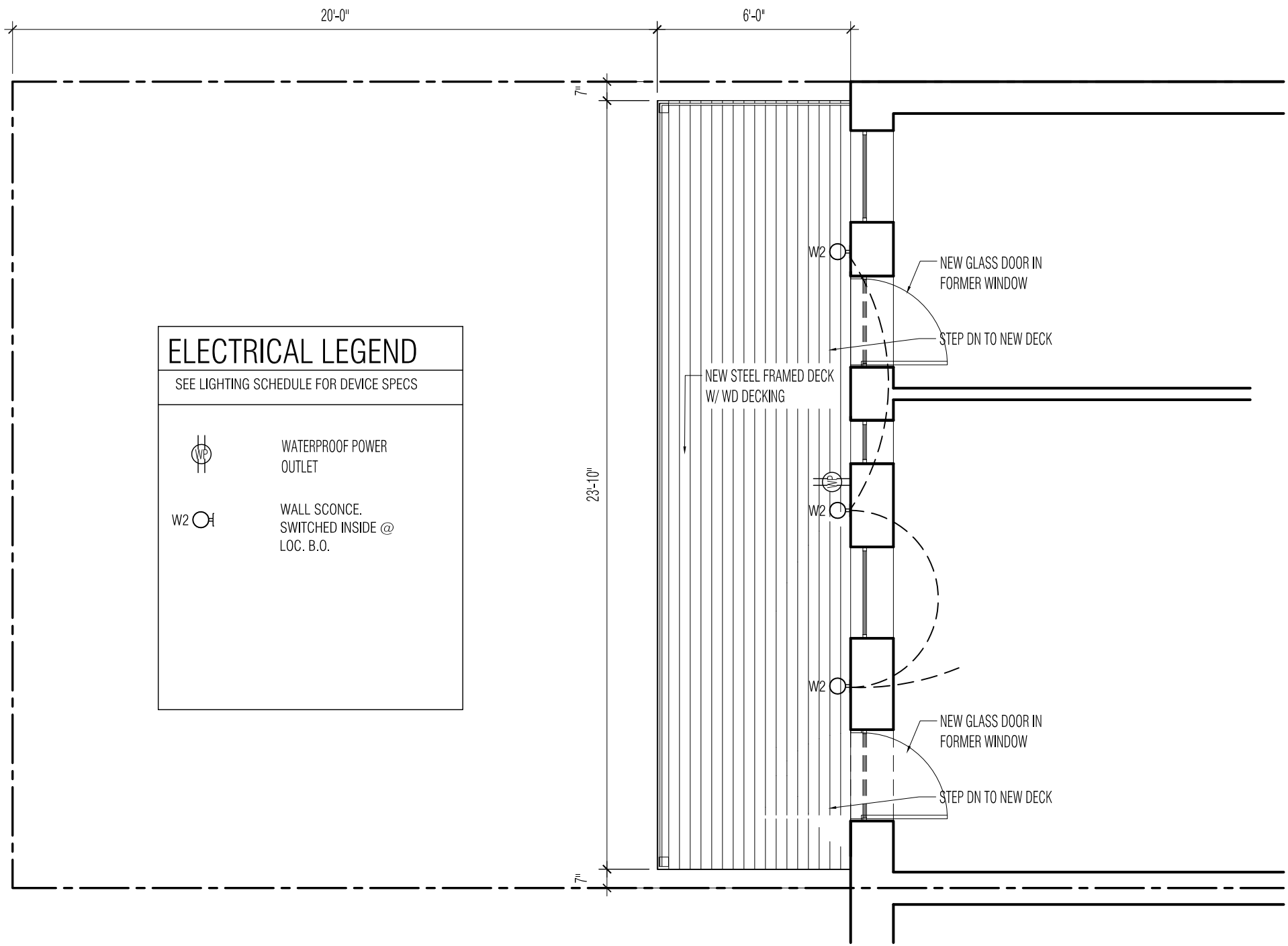
1 SECOND FLOOR PLAN scale: 1/4" = 1'-0"
