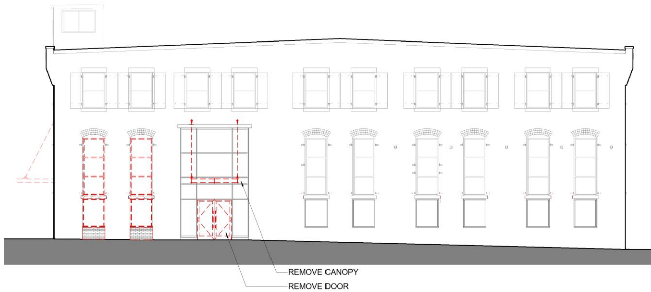
ELEVATION AT PLAZA
