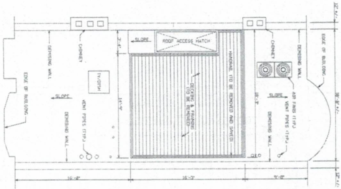
EXISTING DECK DEMOLITION PLAN K-1-B
