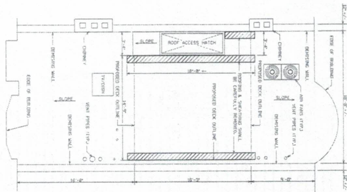
ROOF DEMOLITION PLAN K-1-B
