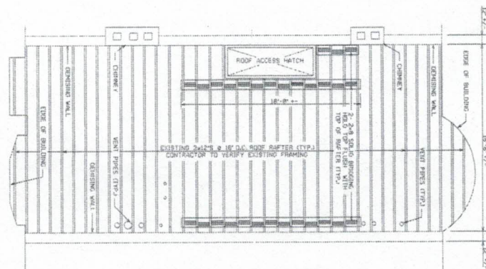
ROOF FRAMING STRENGTHENING PLAN K-1-B
