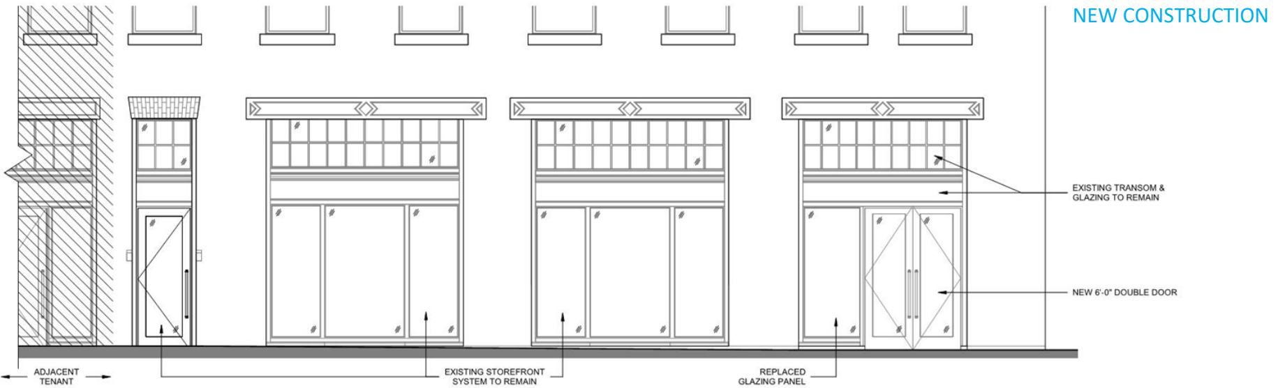
ELEVATIONS OF PROPOSED SCOPE VIEW FACING STILLINGS STREET
