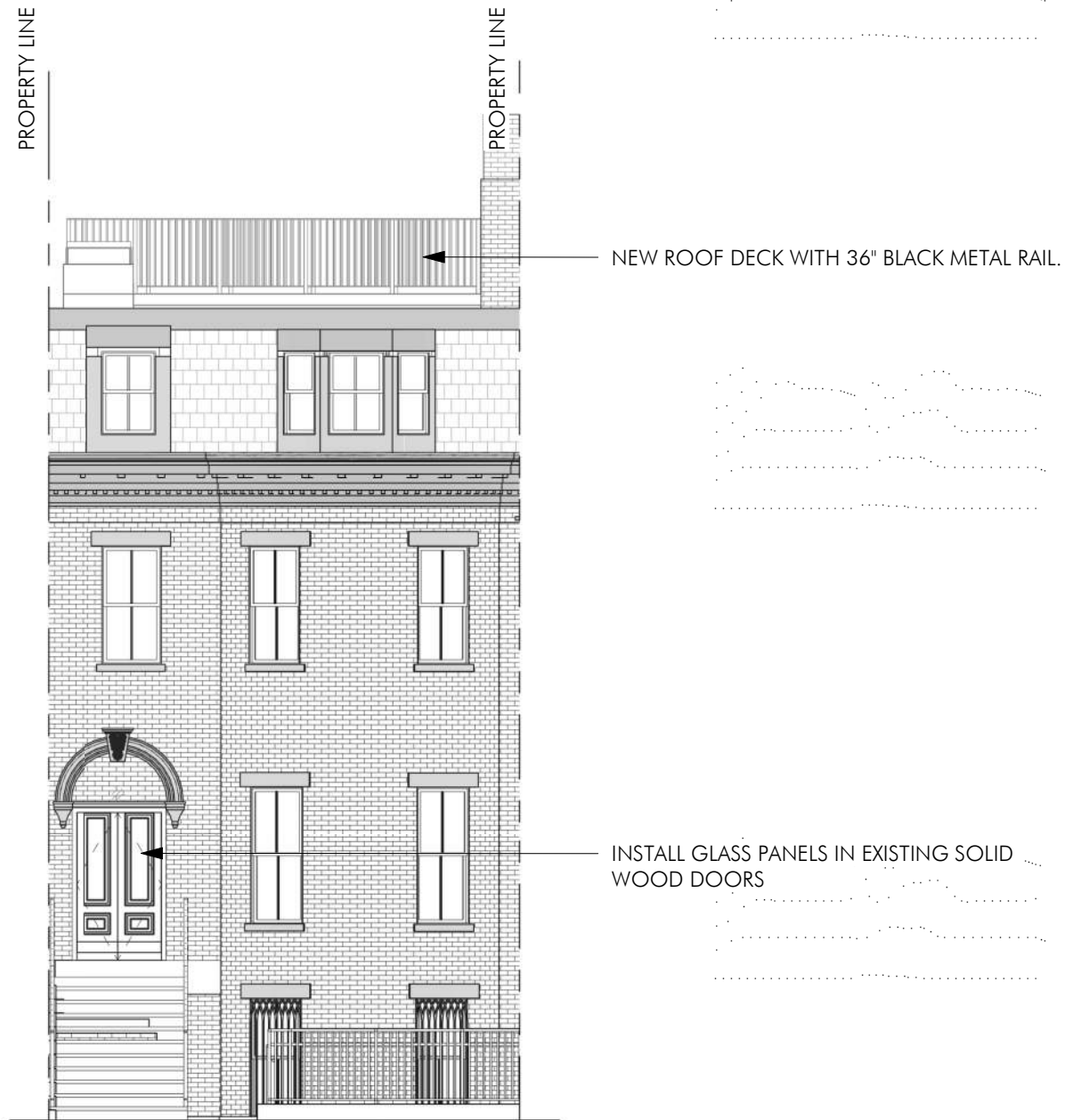
1 PROPOSED FRONT ELEVATION 1/8" = 1'-0"
