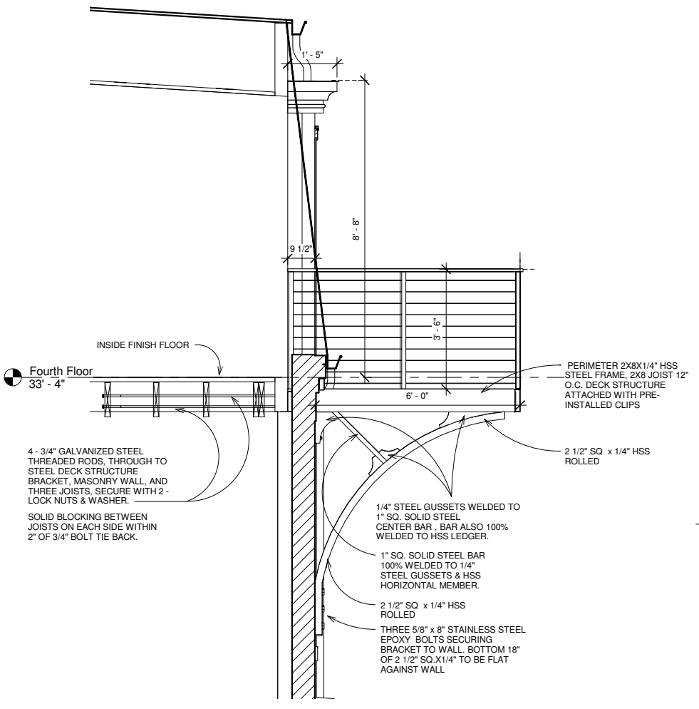
⑤ Section With Deck Structure 1/2" = 1'-0"
