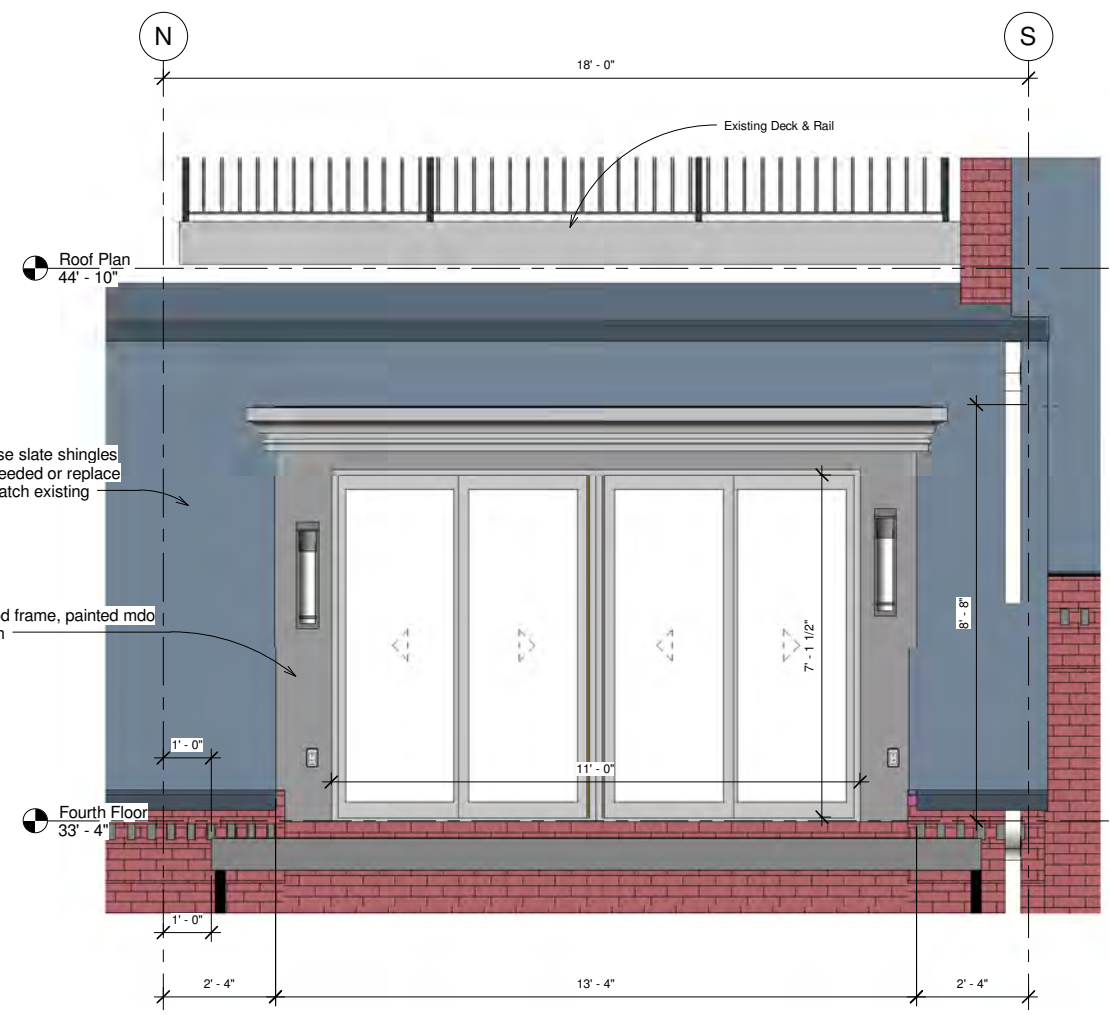
④ Rear Top Floor dormer 1/2" = 1'-0"
