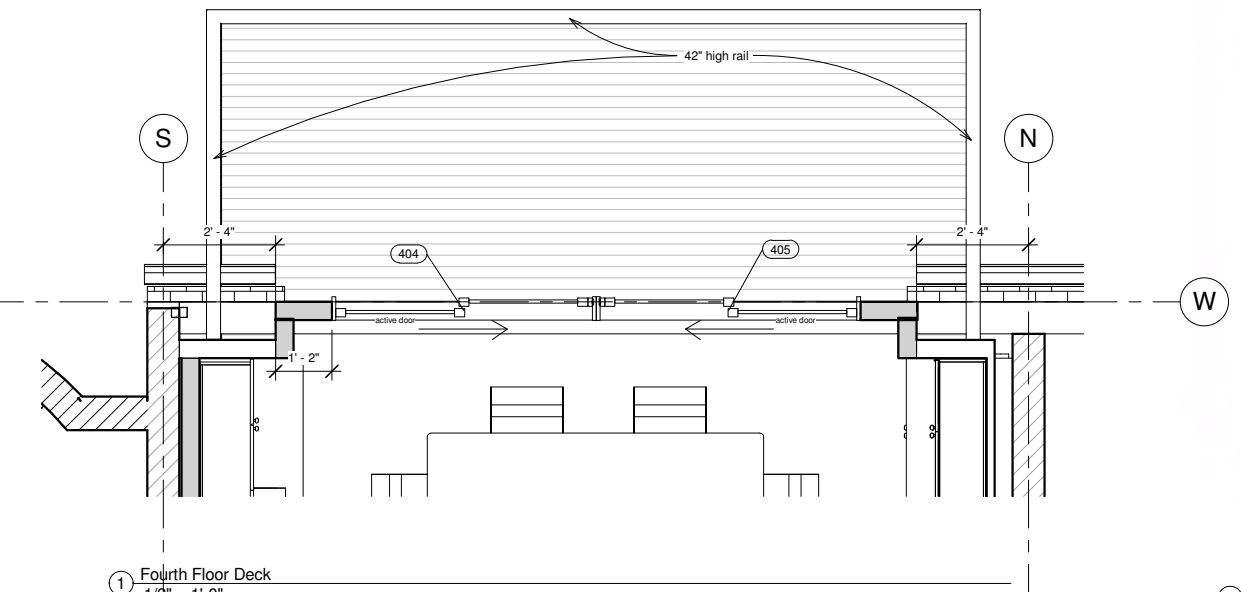
① Fourth Floor Deck 1/2" = 1'-0"
