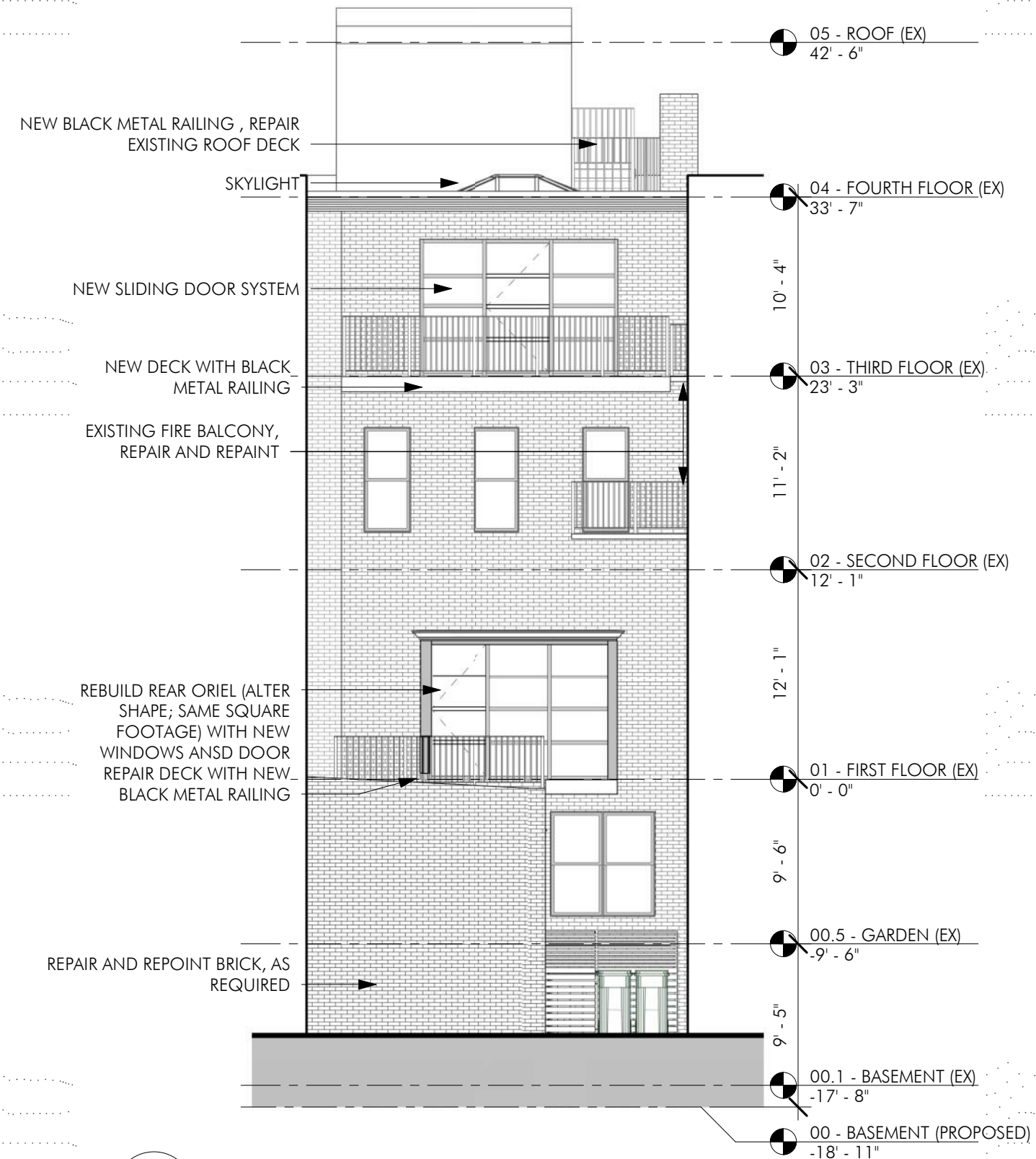
2 REAR ELEVATION - LANDMARKS 1/8" = 1'-0"
