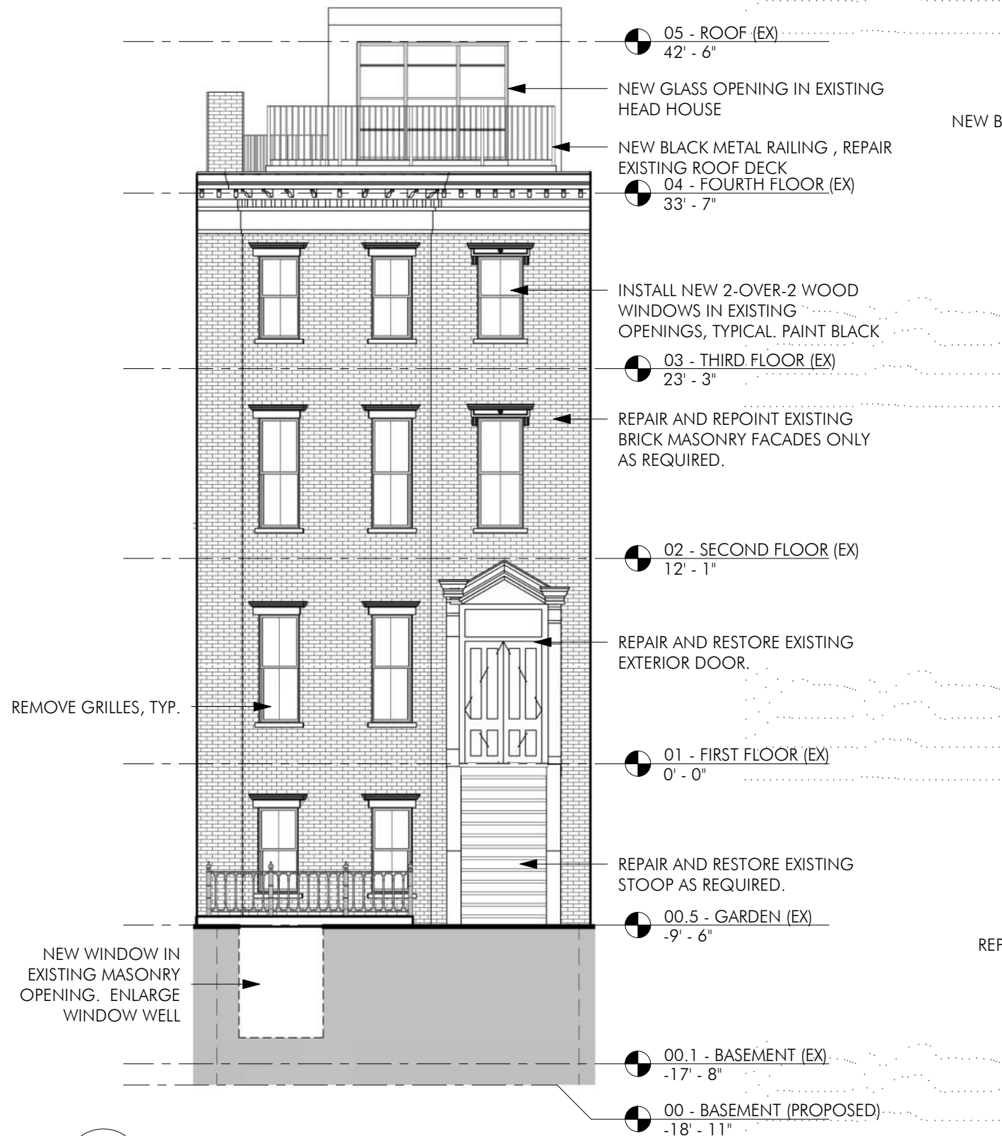
1 FRONT ELEVATION - LANDMARKS 1/8" = 1'-0"
