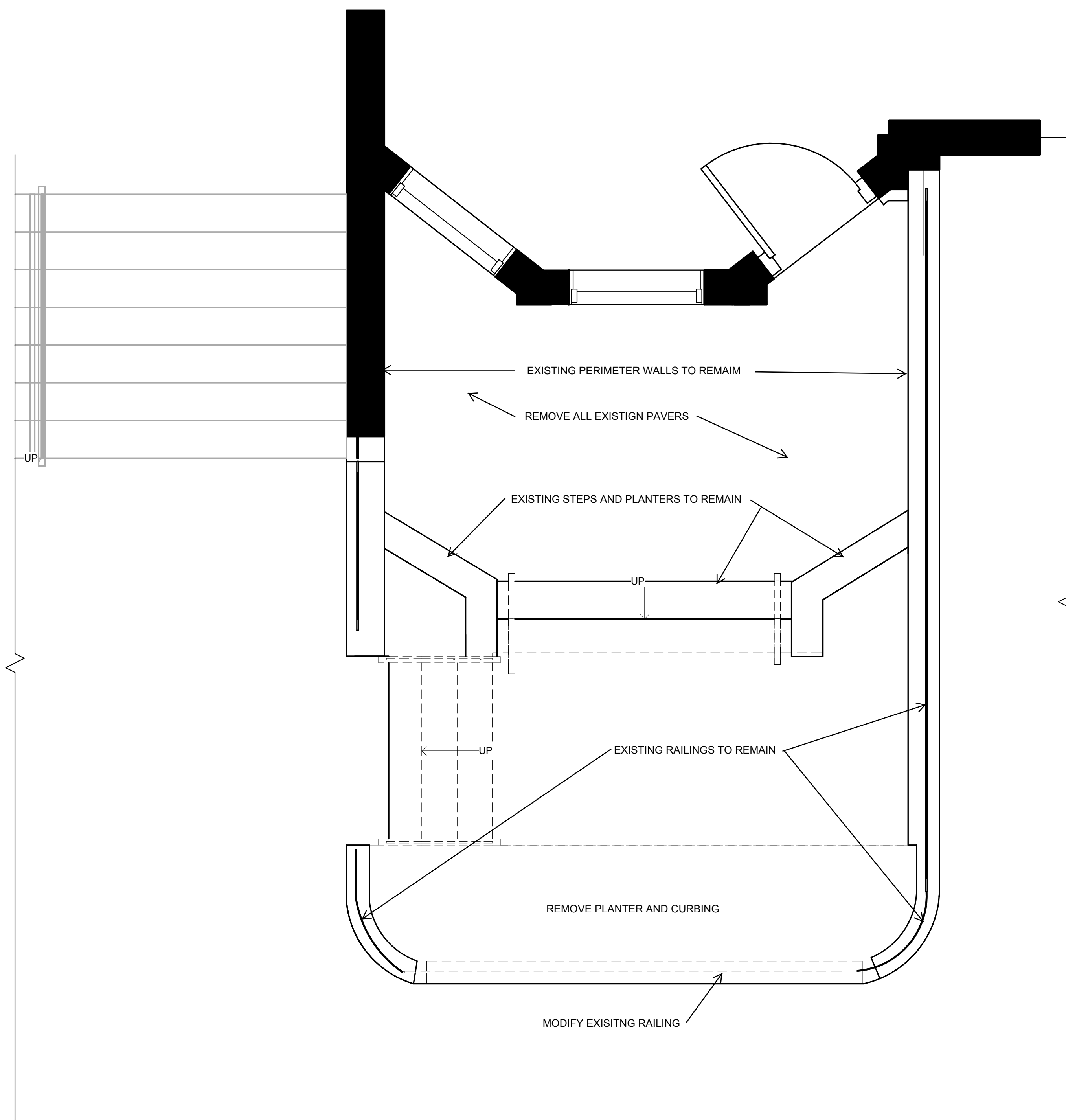
1 D01 - DEMOLITION GARDEN PLAN 1/2" = 1'-0"
