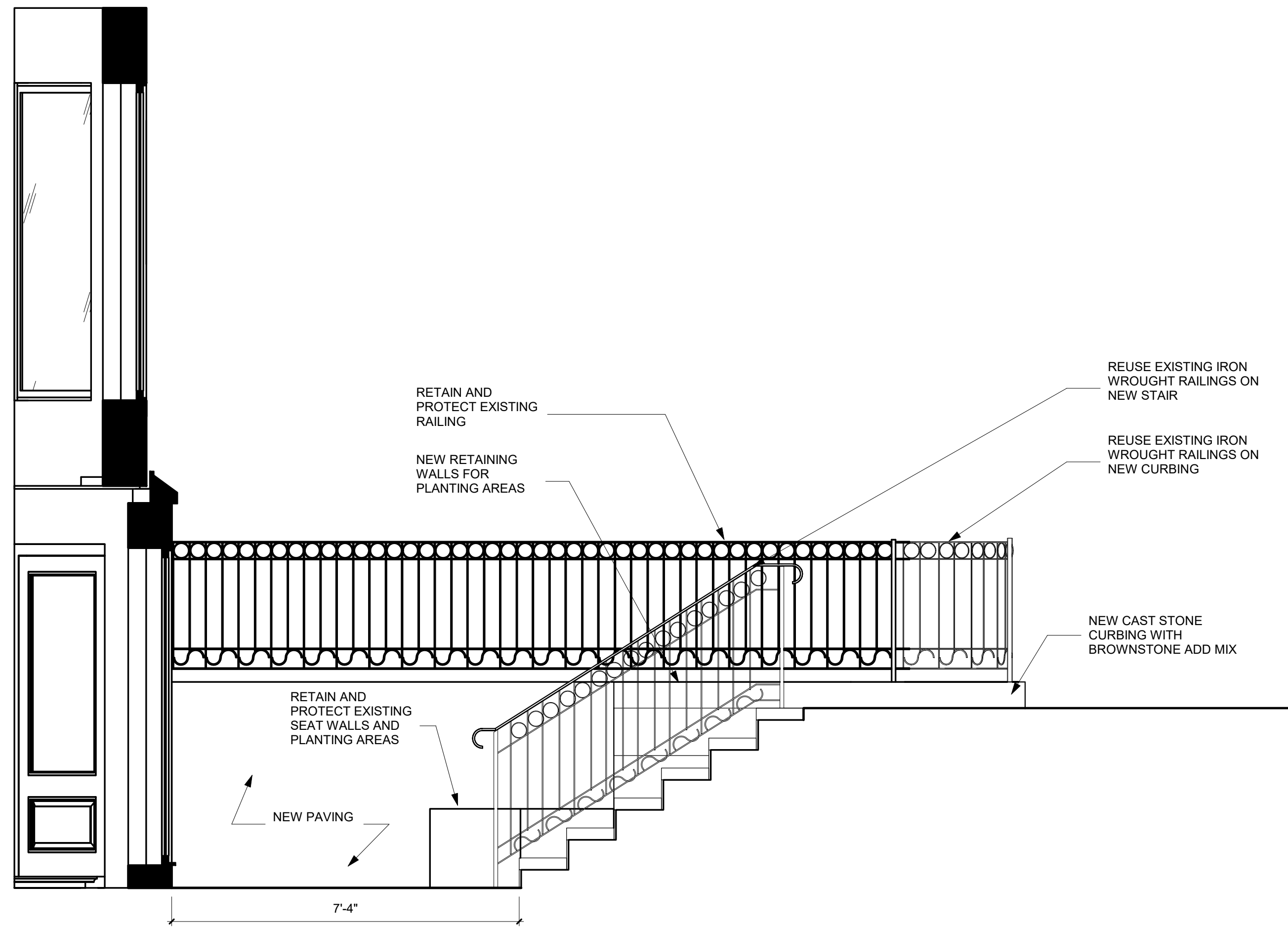
4 SECTION1 1/2" = 1'-0"
