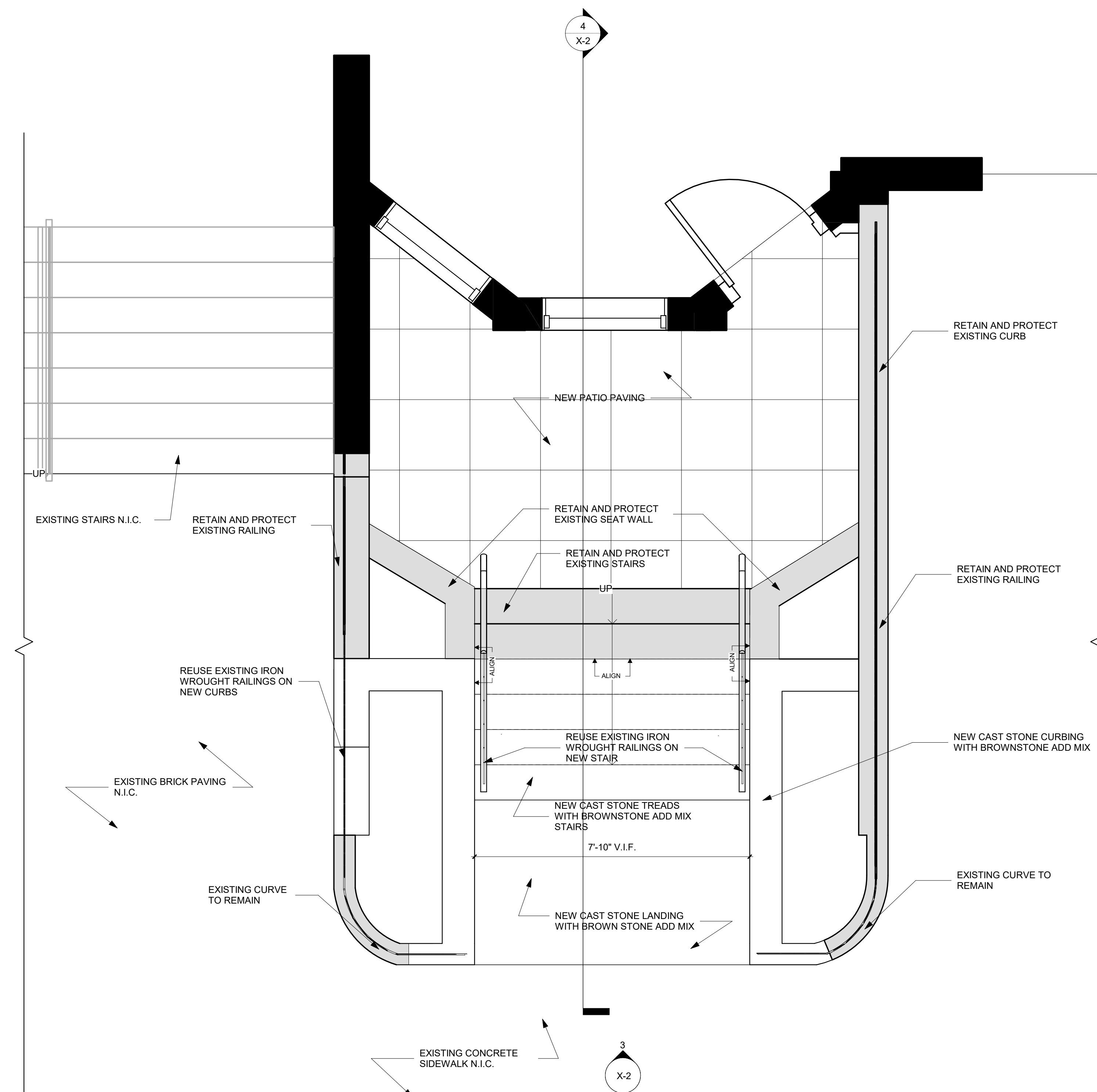
2 01 PROPOSED GARDEN PLAN 1/2" = 1'-0"
