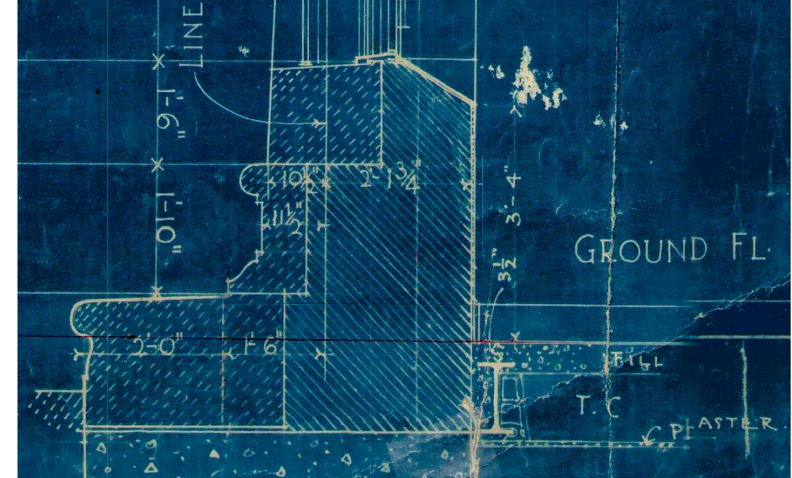
ENLARGED STONE BENCH DETAIL AT TERRACES 1920 ARCHITECT'S DESIGN DRAWING FROM PEARL STREET FAÇADE SECTION
