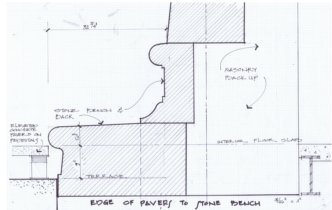
ENLARGED STONE BENCH DETAIL AT TERRACES 1920 ARCHITECT'S DESIGN DRAWING FROM PEARL STREET FAÇADE SECTION
