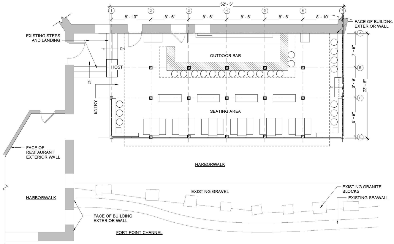
Floor Plan
