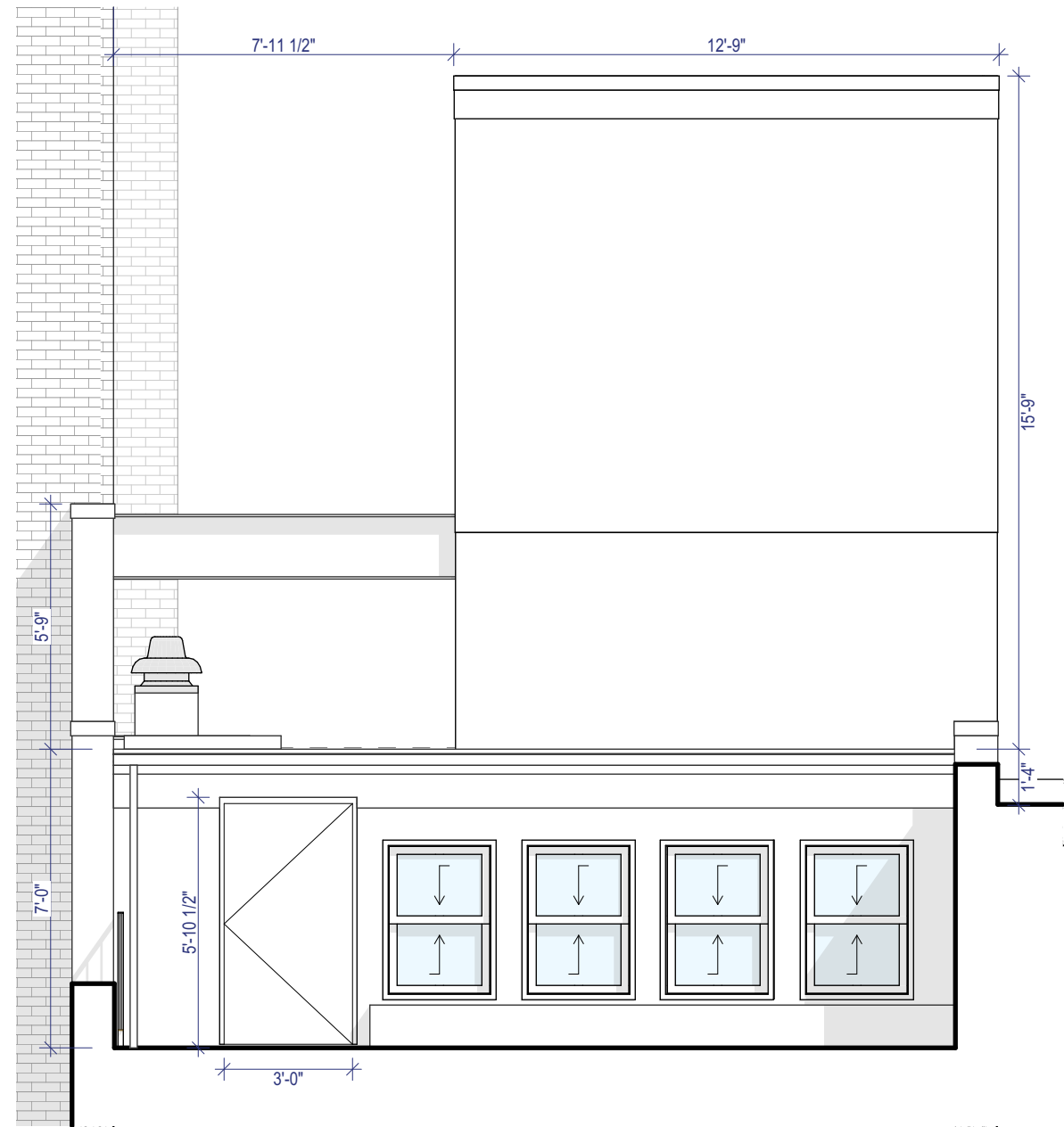
1 Existing Elevation 02 SCALE: 1/4" = 1'-0" 0 2' 4' 8'
