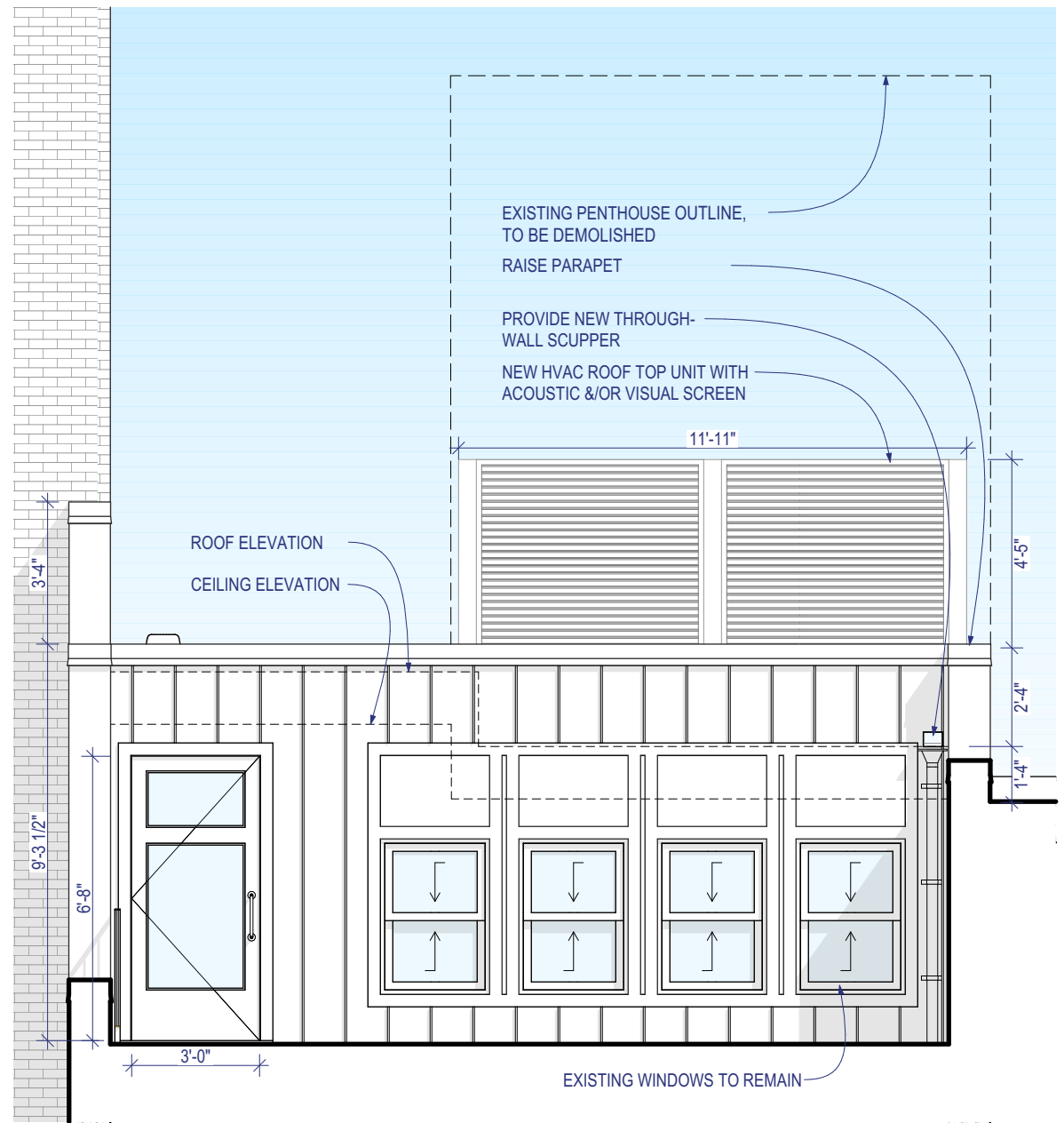
2 Proposed Elevation 02 SCALE: 1/4" = 1'-0" 0 2' 4' 8'
