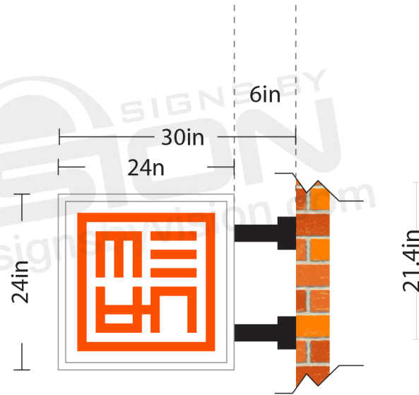
LED Lit Blade Sign | 1x
