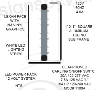
FABRICATED .063 ALUMINUM SIGN CABINET
