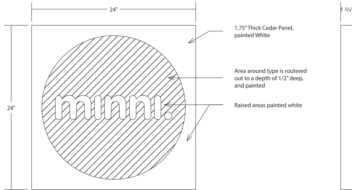
01 FRONT VIEW 3" = 1'-0"
