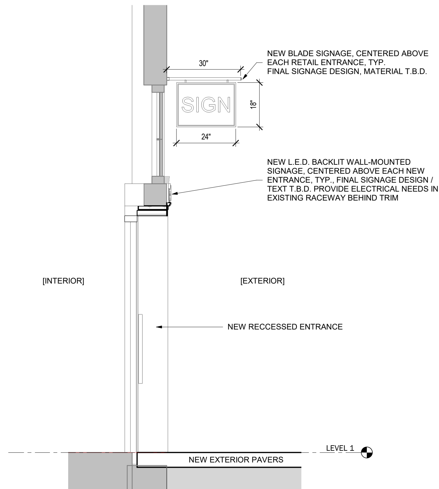
2 SECTION VIEW - SIGNAGE 1/2" = 1'-0"
