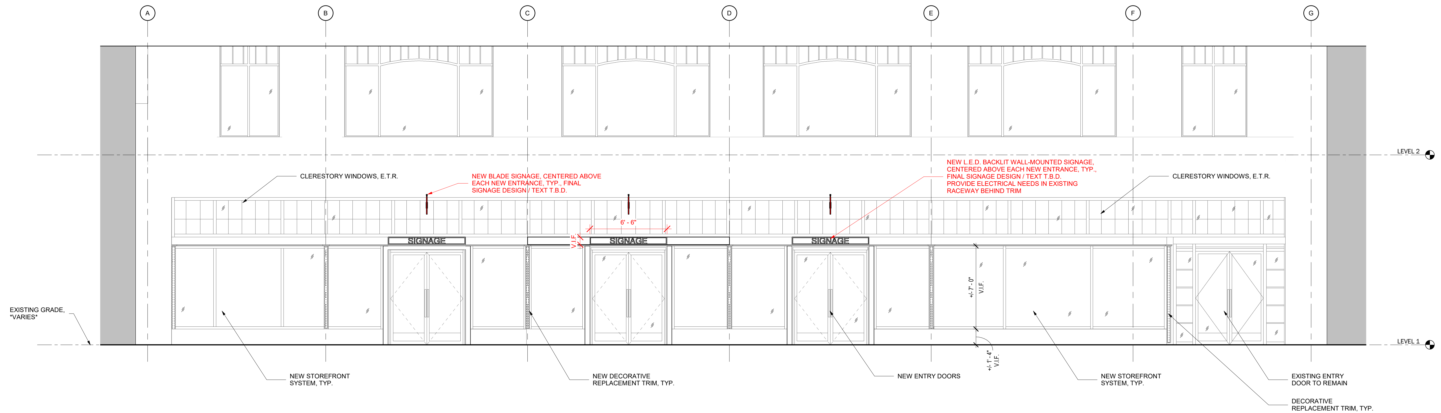
1 ENLARGED ELEVATION @ STOREFRONT - SIGNAGE 1/4" = 1'-0"
