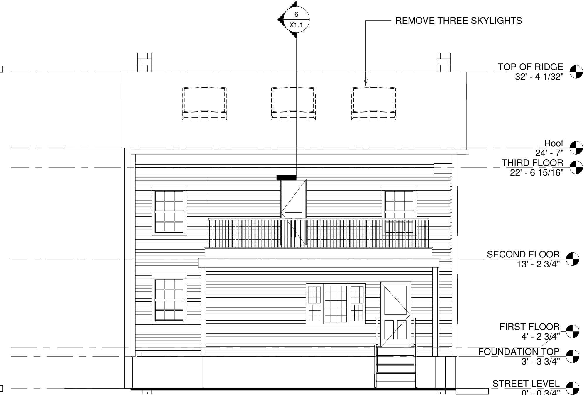
1 NORTH 1 3/16" = 1'-0"
