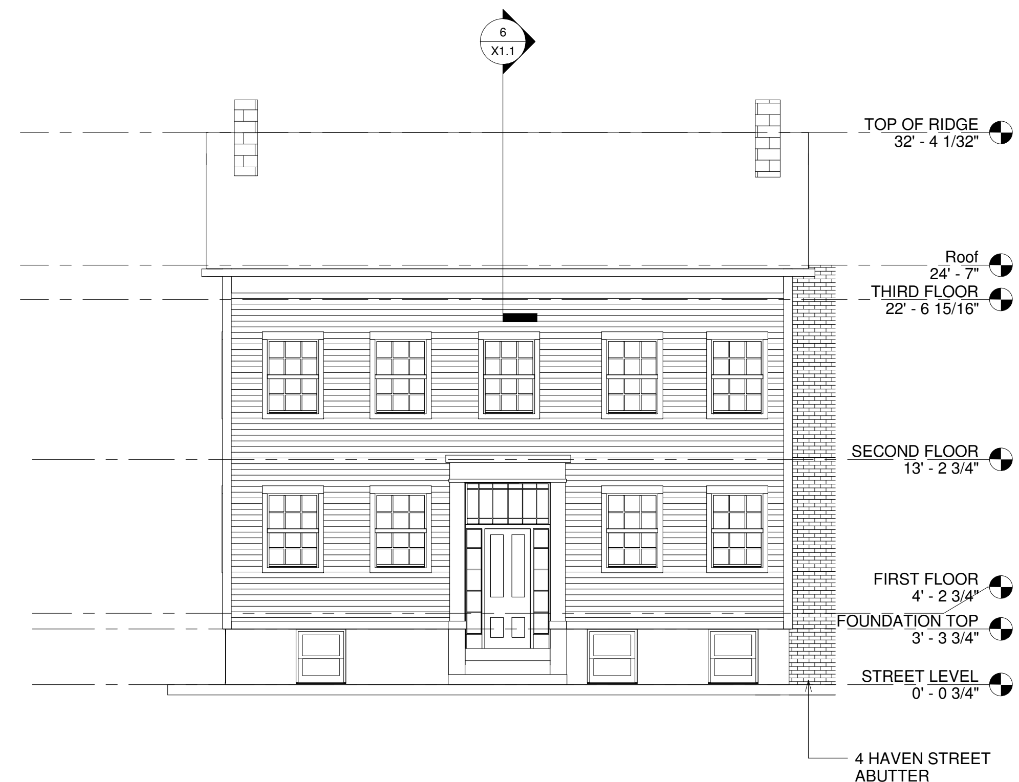
3 SOUTH 3/16" = 1'-0"
