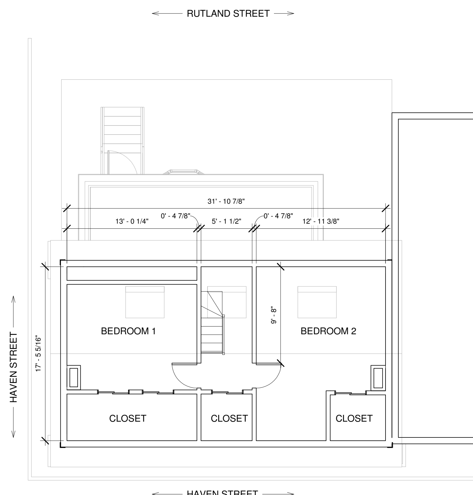
5 THIRD FLOOR 3/16" = 1'-0"
