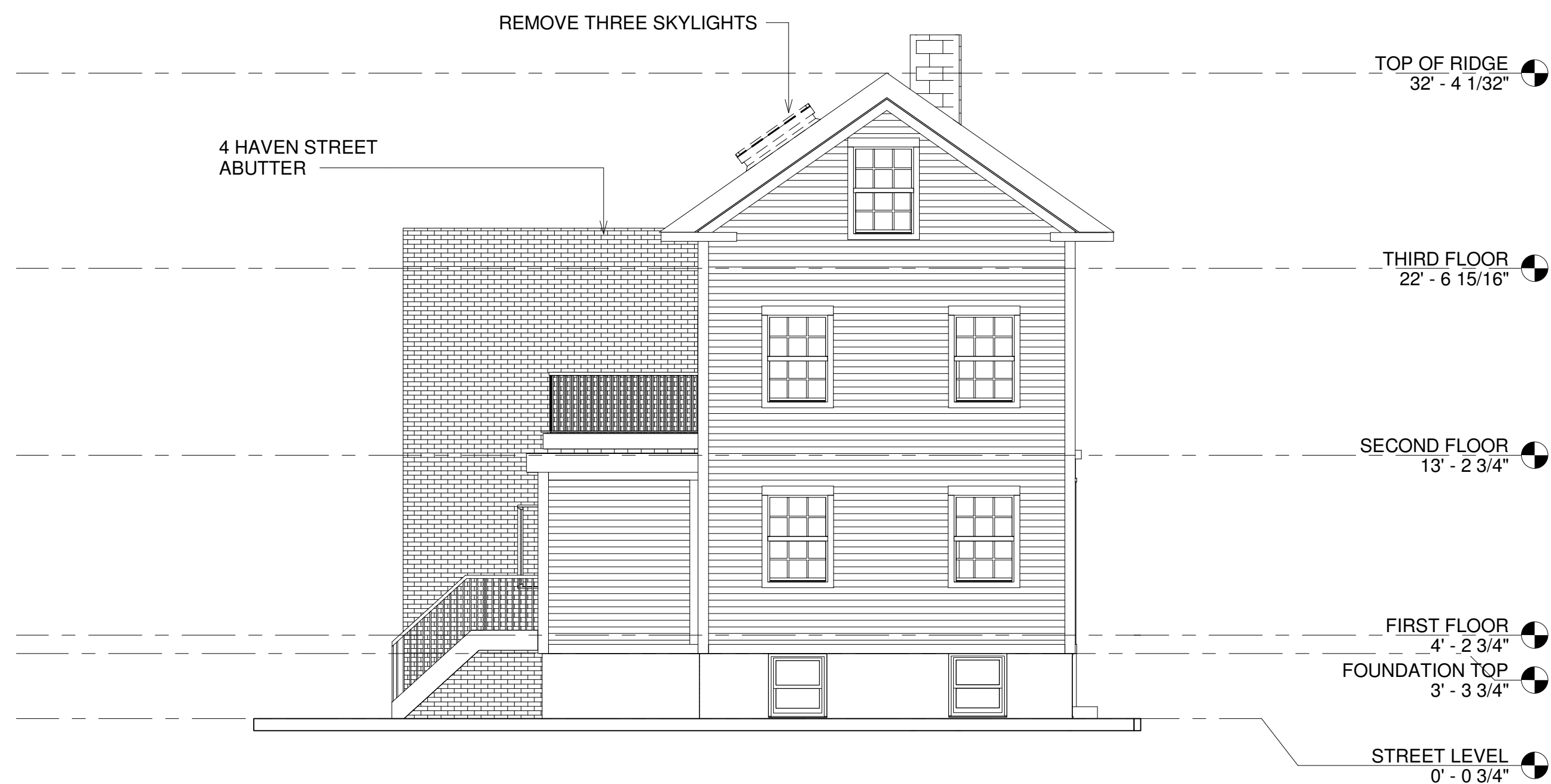
2 WEST 3/16" = 1'-0"
