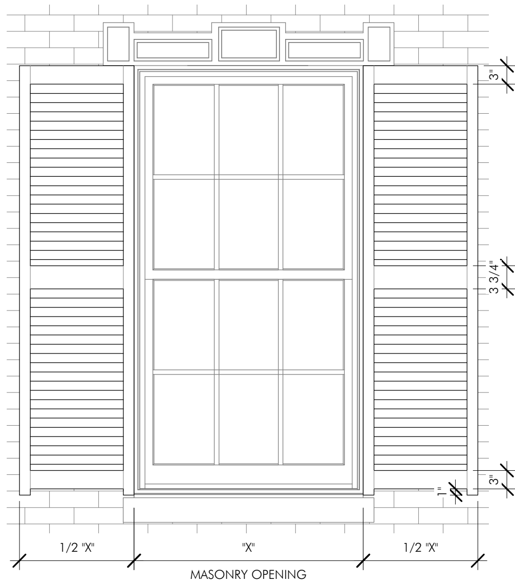
SHUTTER DETAILS
