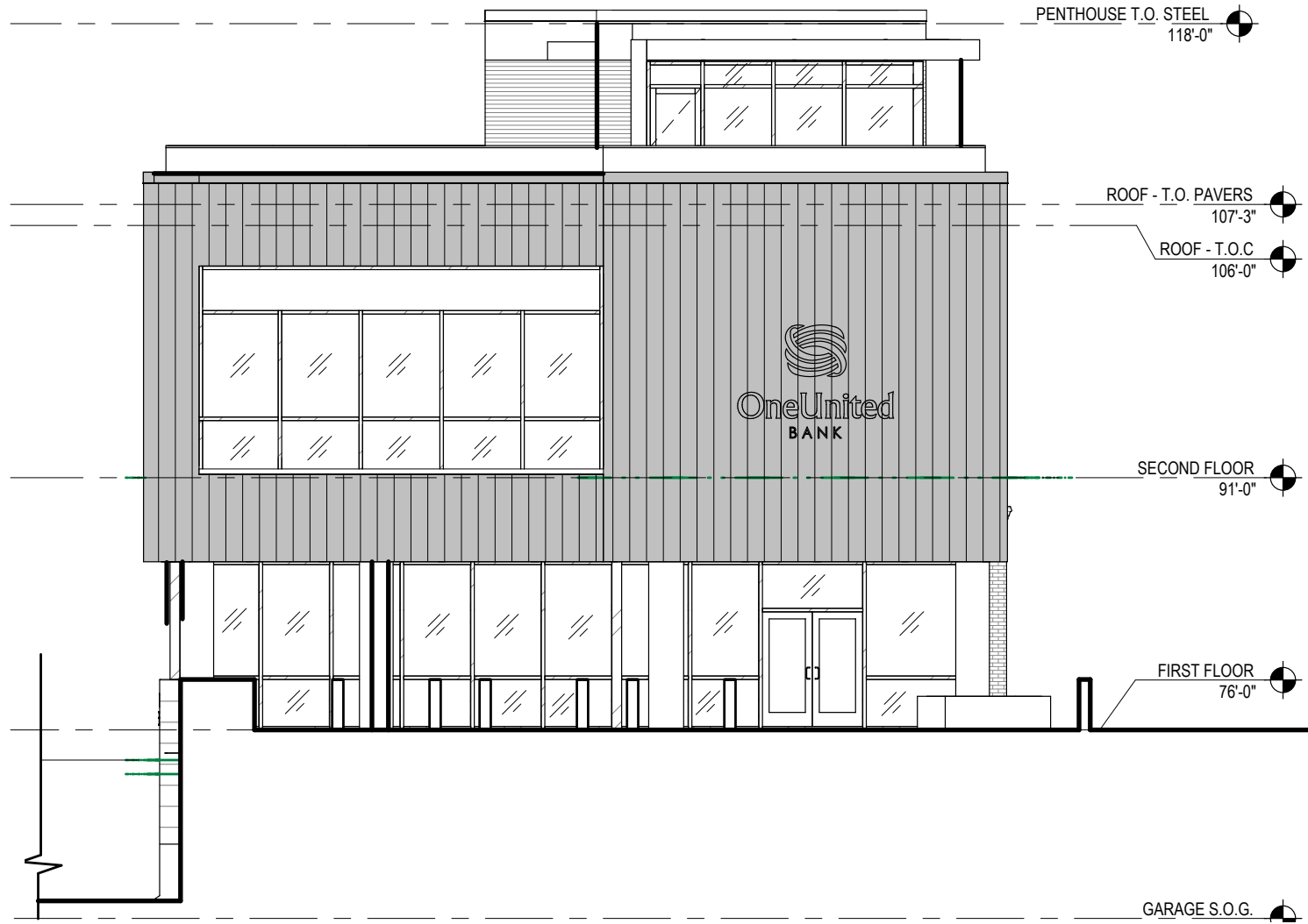
West Elevation
