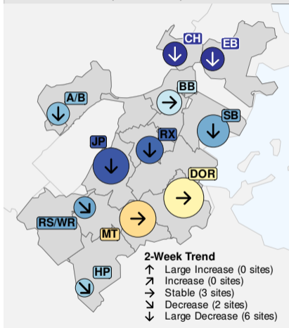
COVID-19 Wastewater Levels & Trends (25-Feb-2024)
