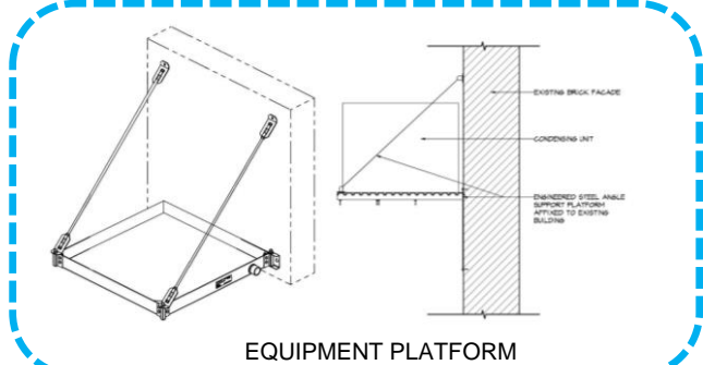
EQUIPMENT PLATFORM
