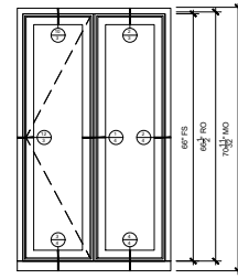
TYPE 1- 4TH FLOOR SCALE: 3/4" = 1'-0"
