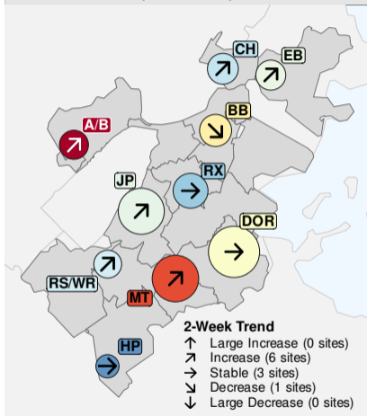
COVID-19 Wastewater Levels & Trends (19-Jun-2024)
