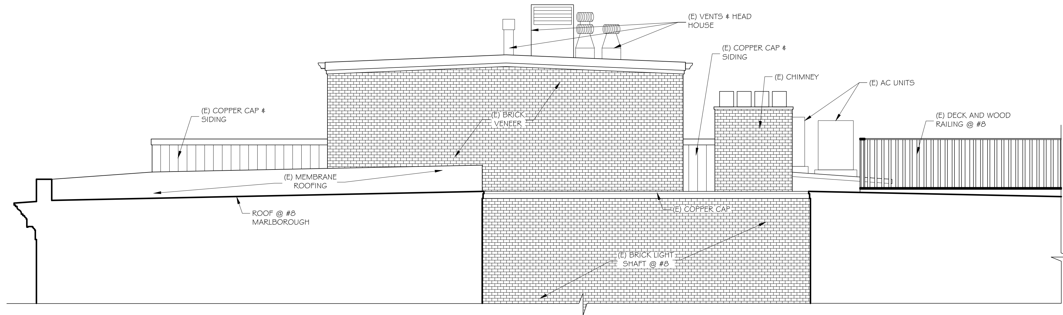
EXISTING SECTION @ #8 MARLBOROUGH / WEST WALL ELEVATION OF #4
