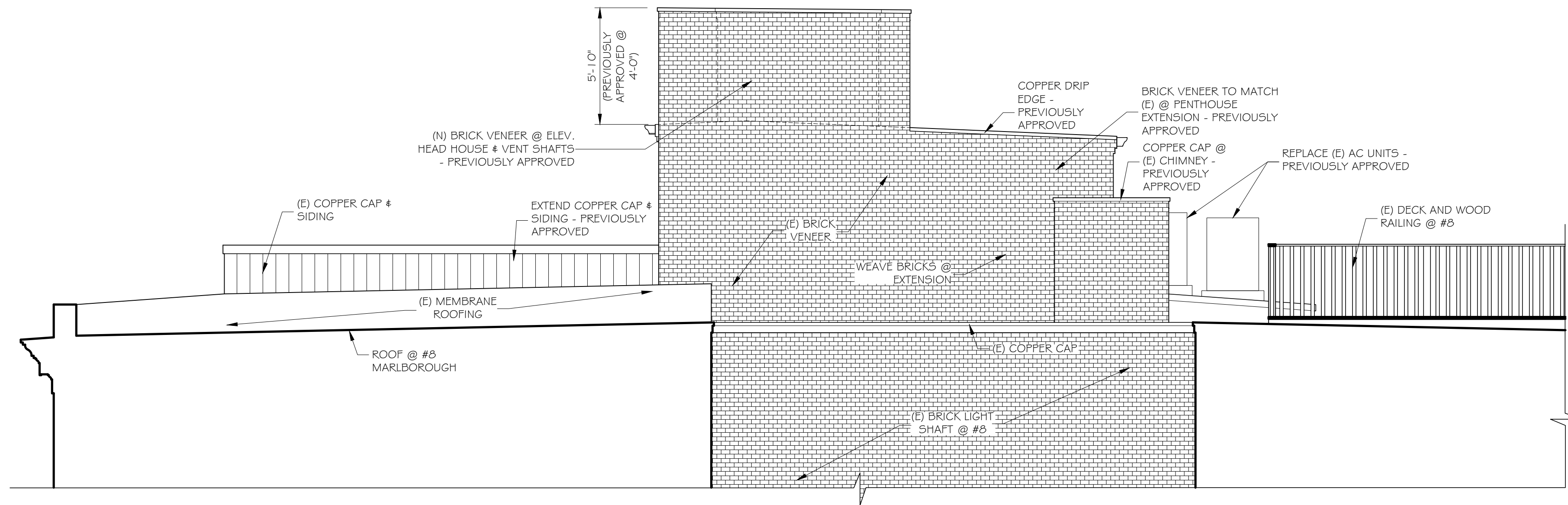
PROPOSED SECTION @ #8 MARLBOROUGH / WEST WALL ELEVATION OF #4
