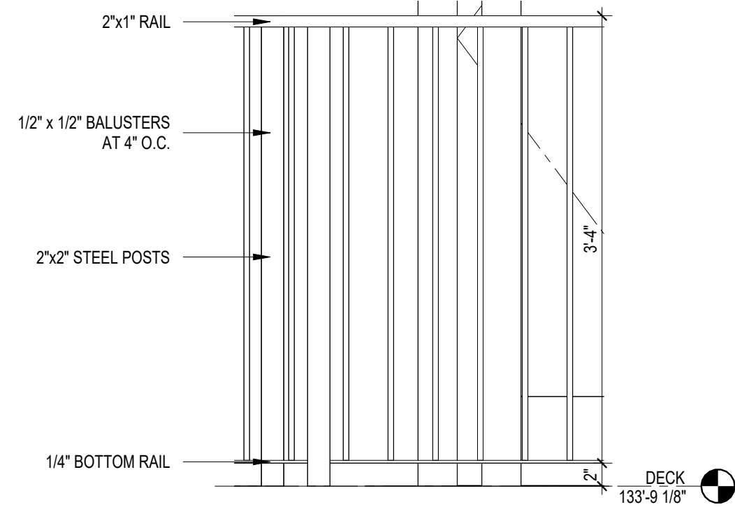
9 RAILING DETAIL 1" = 1'-0"
