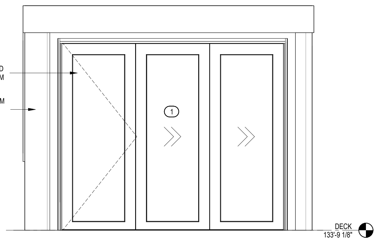
3 SOUTH PROPOSED ELEVATION 1/2" = 1'-0"
