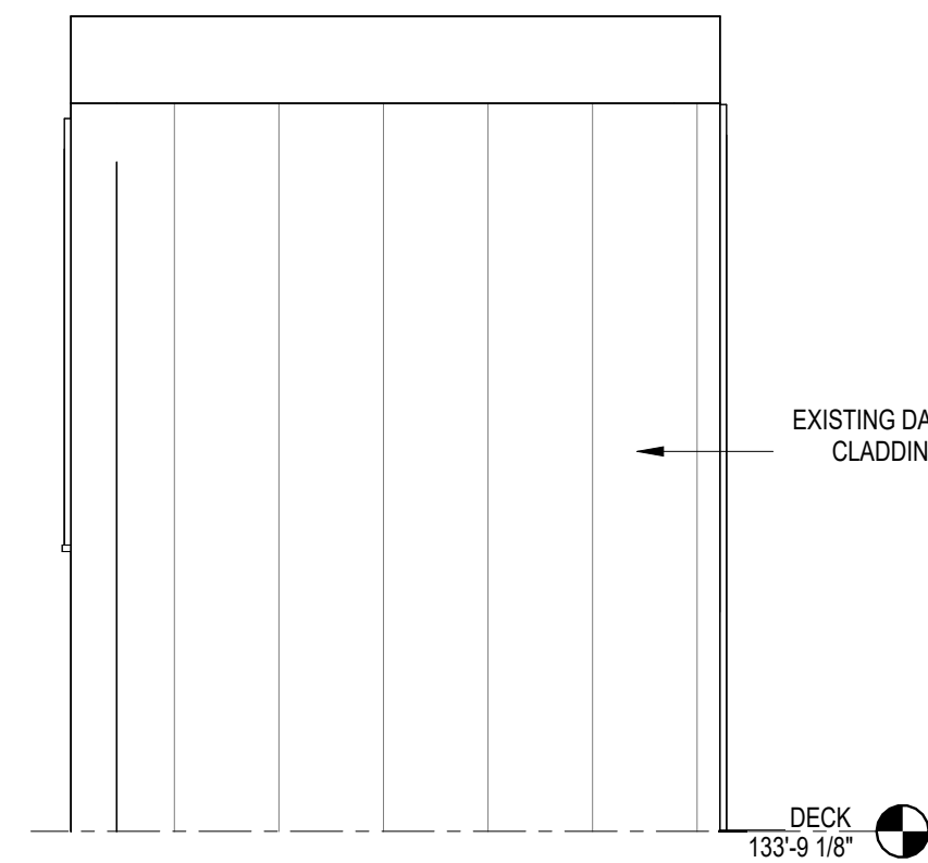
8 EAST EXISTING ELEVATION 1/2" = 1'-0"
