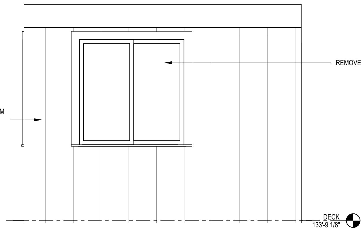
7 SOUTH EXISTING ELEVATION 1/2" = 1'-0"
