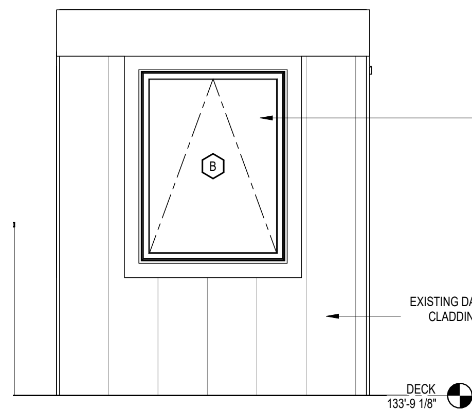
2 WEST PROPOSED ELEVATION 1/2" = 1'-0"
