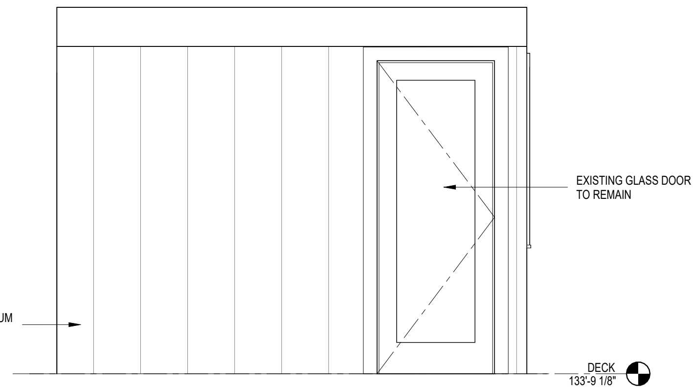
5 NORTH EXISTING ELEVATION 1/2" = 1'-0"
