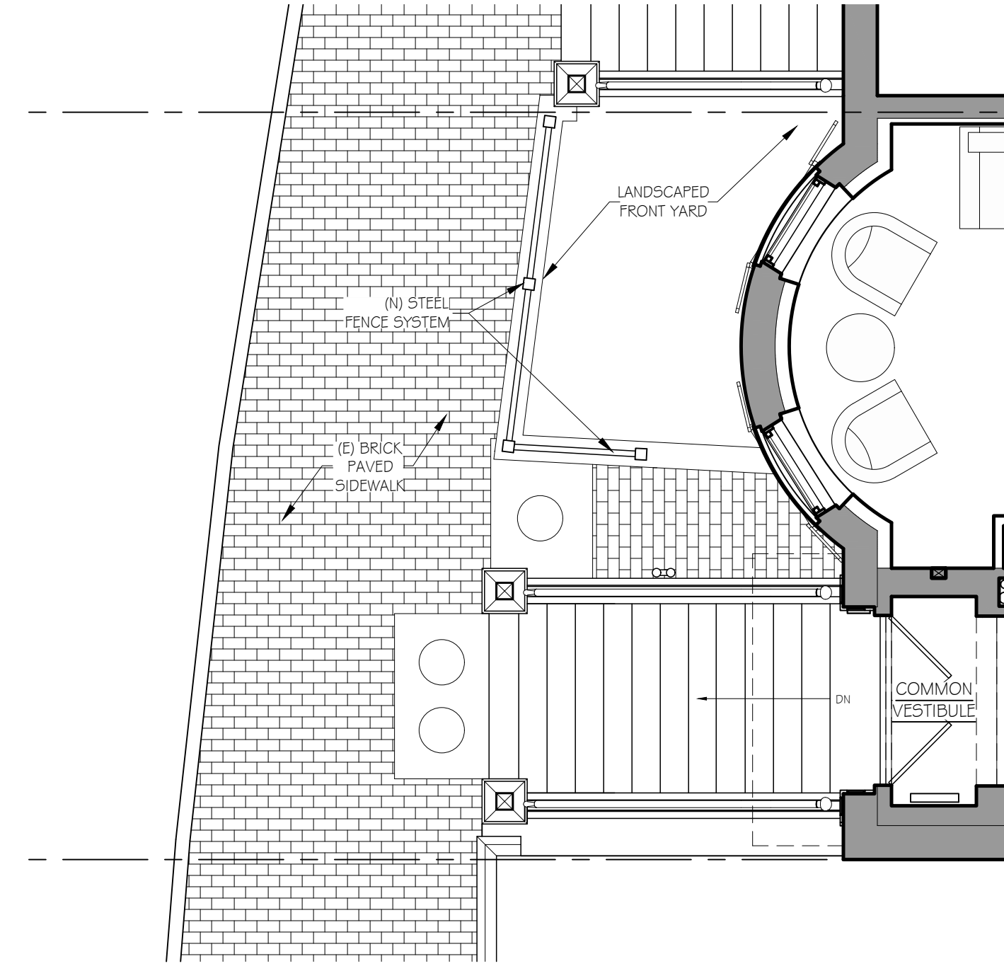
FIRST FLOOR PLAN SCALE: \frac{1}{4}" = 1'-0"
