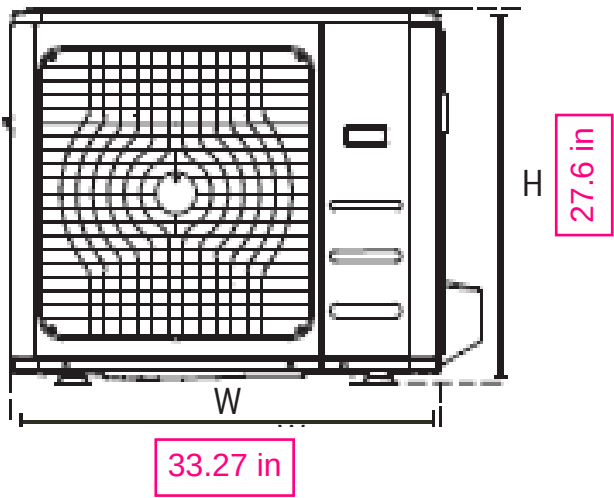
Split Type Outdoor Unit
