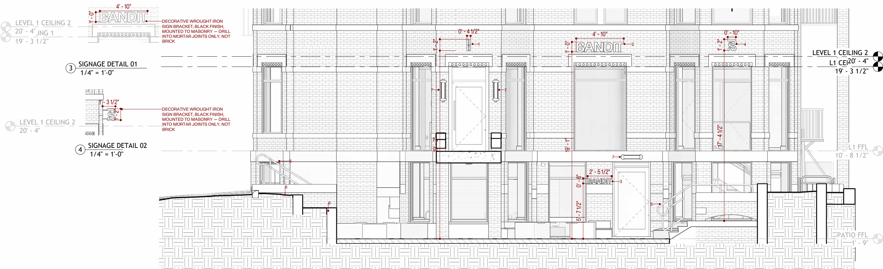
RETAIL LEVEL ENLARGED ELEVATION - EAST 1/4" = 1'-0"
