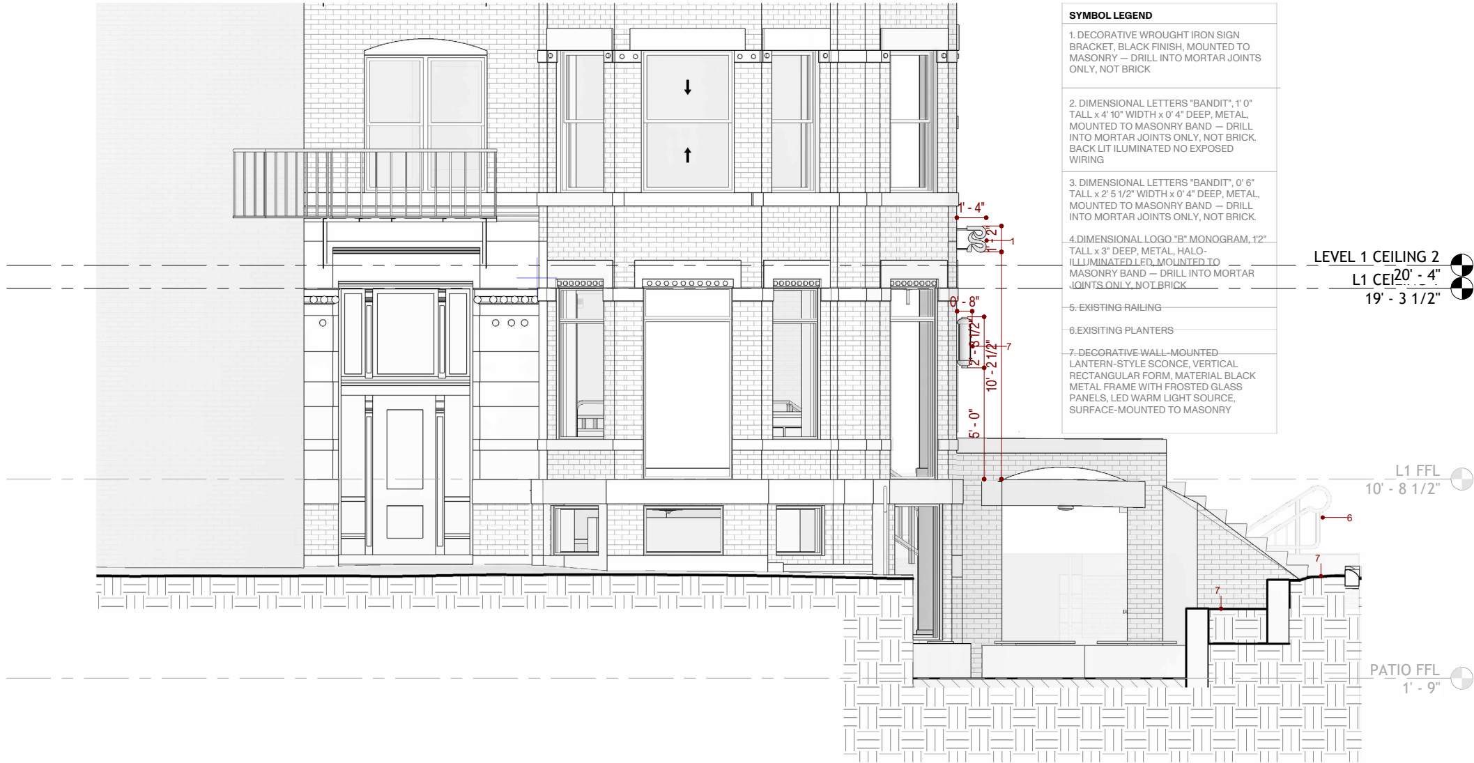
RETAIL LEVEL ENLARGED ELEVATION - WEST 1/4" = 1'-0"
