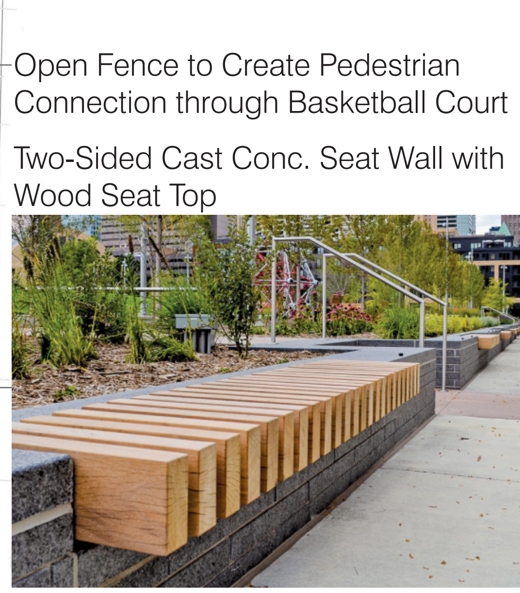
Open Fence to Create Pedestrian Connection through Basketball Court Two-Sided Cast Conc. Seat Wall with Wood Seat Top
